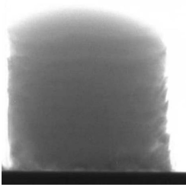
Fig. 3 X-ray image of a sample taken from a 2.5 cm diameter high-porosity dust agglomerate by means of a tube sampler. The diameter of the sample is 7.5 mm. Although the compressive strength of the sample is as low as 500 Pa, the sample structure is preserved at distances \geq 1 mm from the sampler wall
